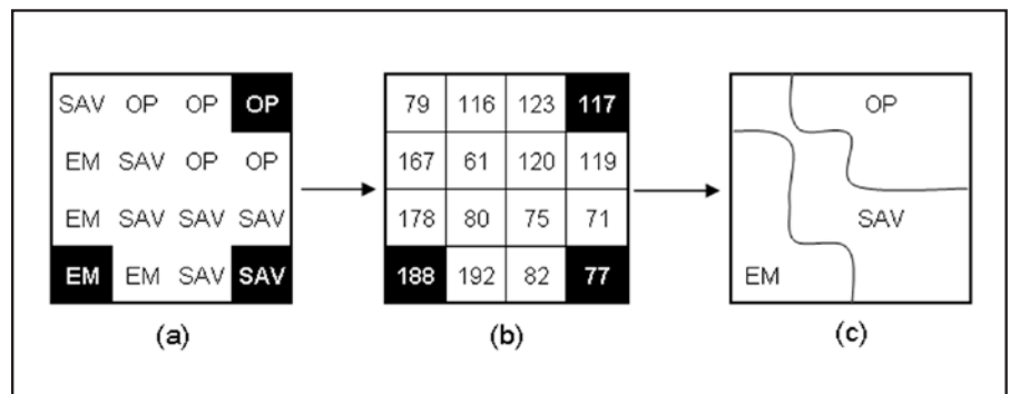
Figure 3. Supervised classification procedure for mapping wetland habitats.
